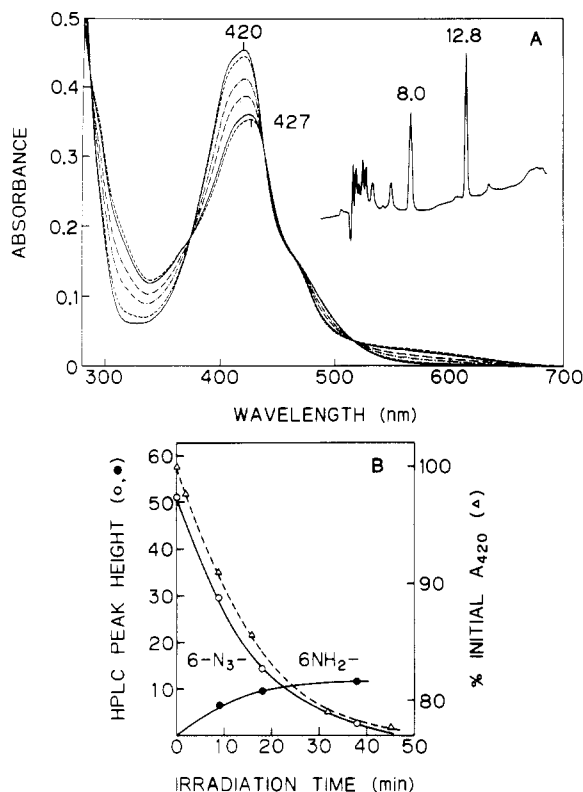
FIGURE 4: (A) Spectral course of photochemical reaction of 6-azido-3-methylumiflavin ( 3a ). 6-Azido-3-methylumiflavin, 2.38 \times 10^{-4} M in 0.1 M phosphate buffer, pH 7.0, was irradiated with a 15-W daylight fluorescent desk lamp (approximately 25 cm from the sample). (—) Starting spectrum. (---), (---), (---), (---), and (---) were obtained after 1.5, 9, 17, 31, and 44 min, respectively. The inset shows the HPLC analysis of a sample obtained after 18-min irradiation. The elution gradient was 0.01 M phosphate buffer, pH 6.0/90% methanol as described under Experimental Procedures. 6-Azido-3-methylumiflavin ( 3a ) elutes at 12.8 min and 6-amino-3-methylumiflavin ( 1a ) after 8.0 min. (B) Concentration dependence of the components of the experiment of (A) on the time of irradiation. ( \Delta ) Absorbance changes at 420 nm; ( \circ ) and ( \bullet ) relative peak height of the signals corresponding to 6-azido- and 6-amino-3-methylumiflavin, respectively, obtained from HPLC elution profiles such as that shown in the inset of (A).
