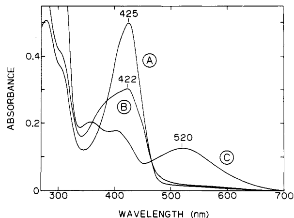
FIGURE 6: Spectral course of Cu^{2+} complexation of 3,8-dimethyl-6-carboxy-7-(2-methyl-3-oxobut-2-enyl)lumazine ( 8a ). The compound, 100 \mu L of a stock solution in dimethyl sulfoxide containing 0.3% acetic acid, was diluted into 1.0 mL of 0.1 M acetate buffer, pH 5.0 (curve A). A total of 20 \mu L of a 0.5 M solution of Cu(NO_3)_2 in the same buffer was then added to generate the spectrum of curve B. Addition of a small amount of solid dithionite led to formation of the spectrum of curve C. Upon being mixed with air, a spectrum identical with that of curve C of Figure 5 was obtained.
