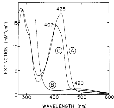
FIGURE 5: Spectral properties and redox reaction of 3,8-dimethyl-6-carboxy-7-(2-methyl-3-oxobut-2-enyl)lumazine ( 8a ). The product from acid degradation of 6-azido-3-methylumiflavin ( 3a ) was dissolved in dimethyl sulfoxide containing 0.3% acetic acid and then diluted 20-fold in 0.1 M acetate buffer, pH 5.0 (curve A). To this a grain of solid dithionite was added, and spectrum B was recorded after careful mixing. Admission of air generated the spectrum of curve C. Repetition of the dithionite/air cycles generates the species of curves B and C.
