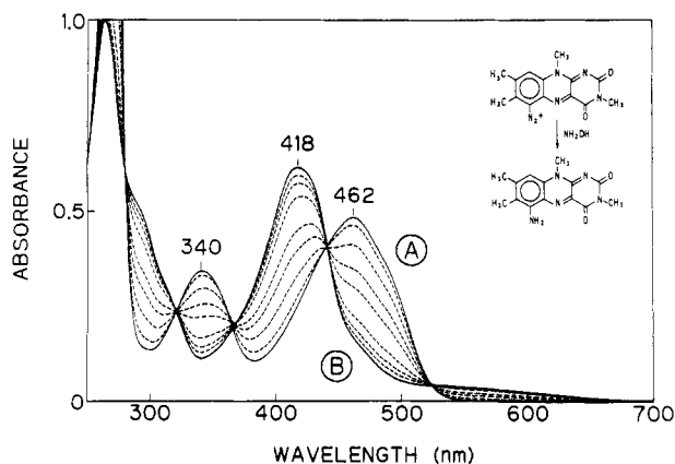
FIGURE 2: Absorption spectrum of 3-methylflavin 6-diazonium cation ( 2a ) and conversion to 6-amino-3-methylflavin ( 1a ). A total of 50 \mu L of a stock solution of 2a in acetonitrile containing 1% \text{CH}_3\text{COOH} was diluted into 950 \mu L of dilute acetic acid (pH 2.5) (curve A). A 50- \mu L aliquot of 1 M \text{NH}_2\text{OH}\cdot\text{HCl} was then added, and the following curves were recorded after approximately 1, 4, 8, 12, 22, 32, and 42 min. The final spectrum (curve B) is identical with that of 6-amino-3-methylflavin ( 1a ) under the same conditions and was obtained after 80 min.
