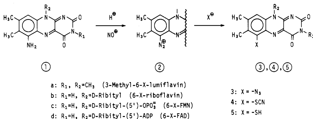
Scheme I: Structures of 6-Substituted Flavins at Lumiflavin, Riboflavin, FMN, and FAD Levels
