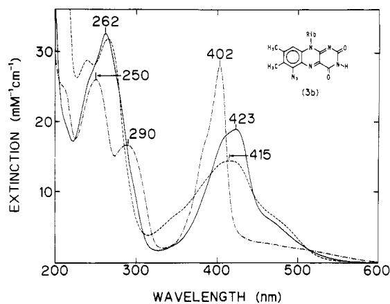
FIGURE 3: Spectra of 6-azidoriboflavin ( 3b ) and pH dependence. Aliquots (50 \mu L) of 6-azidoriboflavin in dimethylformamide were diluted with 1 mL each of 0.1 M phosphate, pH 6.0 (—), 50 mM NaOH (---), or 20% \text{HClO}_4 (-·-·-). Extinction coefficients were determined by titration of 6-azidoriboflavin at pH 7.0 with a standardized solution of riboflavin-binding protein (see text for details).
